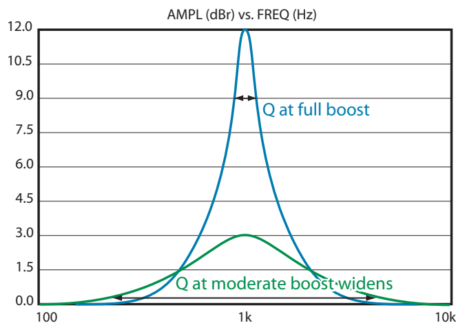
Figure 3. Conventional Graphic
