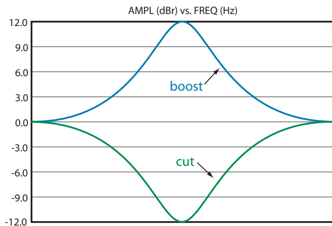
Figure 2. Typical Equalizer Response
