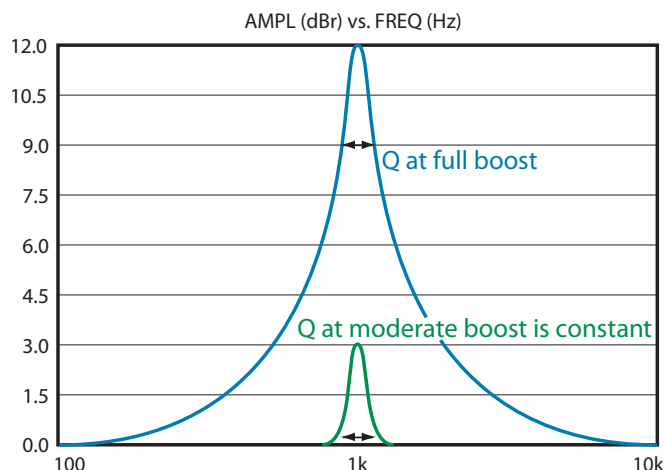
Figure 4. Constant-Q Graphic
