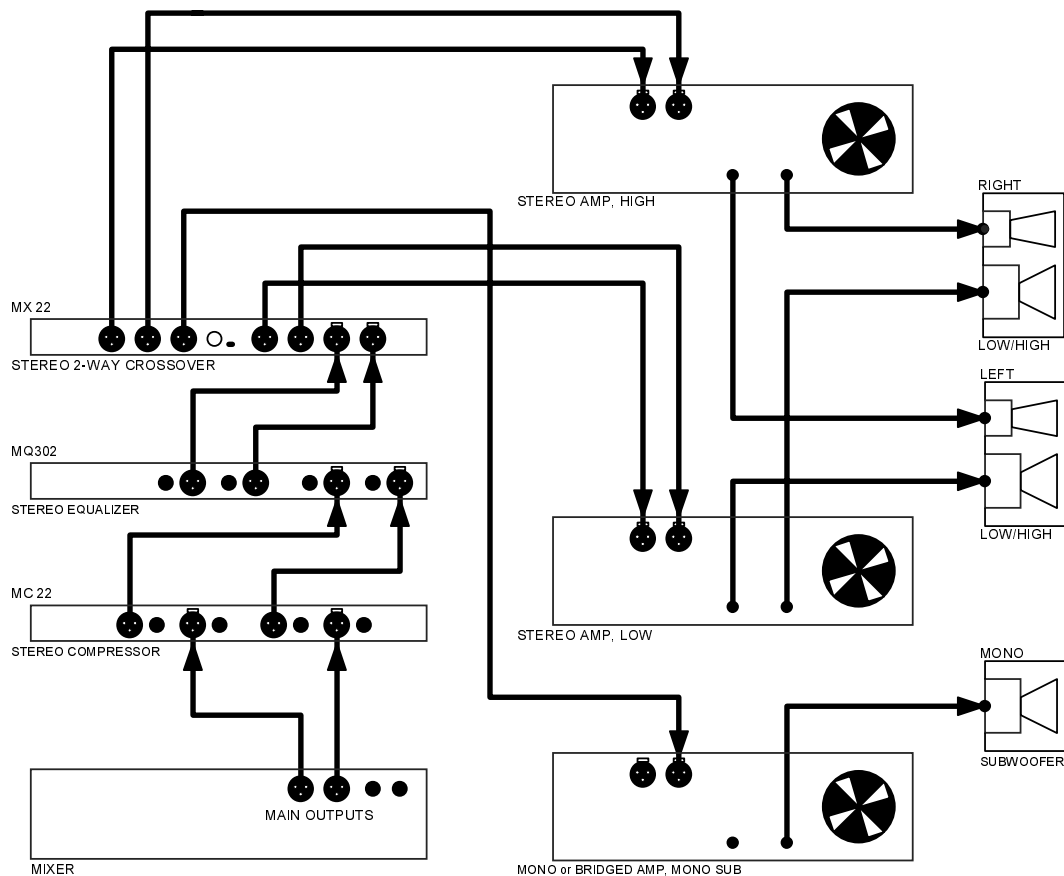
Figure 1. Stereo Biamp System with Equalizer
