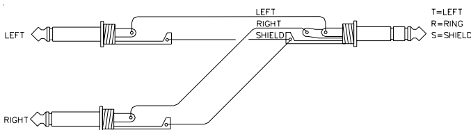
Figure 1. Dual Mono to Stereo TRS Wye Cable.
