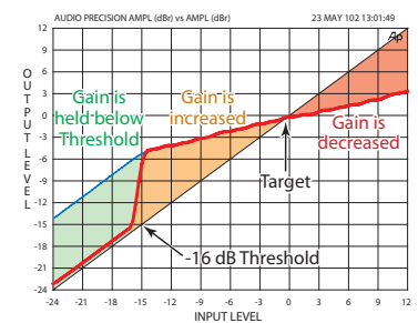
Automatic Gain Control (input level decreasing)
