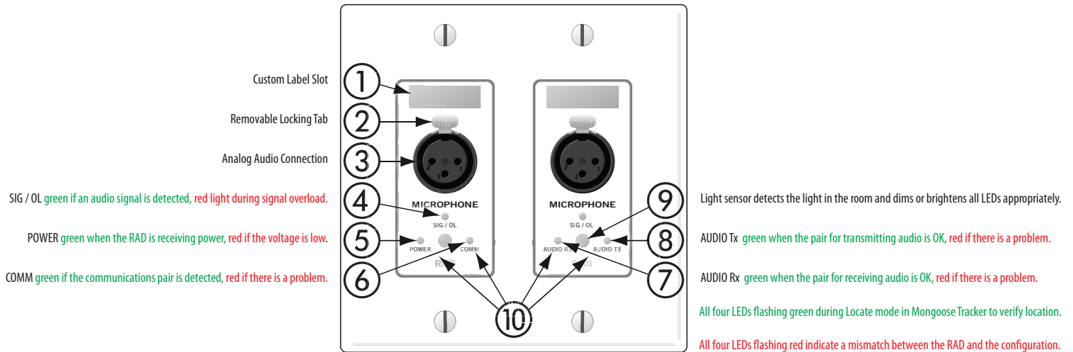
Figure 7: Remote Audio Device
