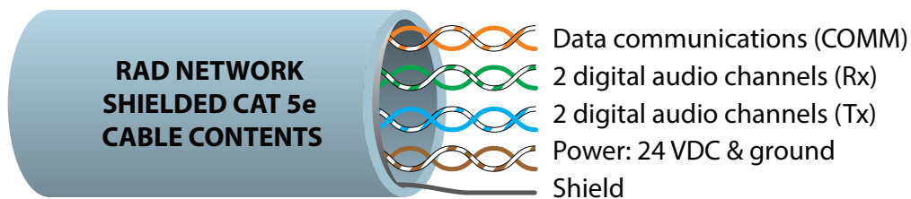
Figure 4: Purpose of each shielded CAT 5e twisted pair
