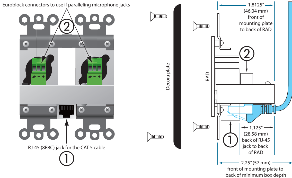
Figure 6: Behind a RAD
