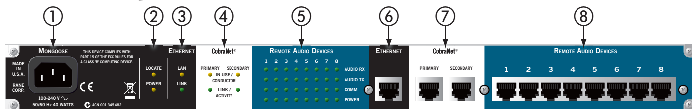
Figure 2: Rear panel of the Mongoose
